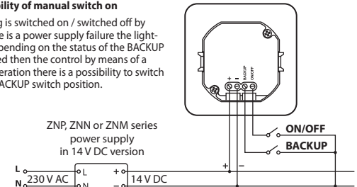
Figure 2. Battery backup with a possibility of manual switch on
