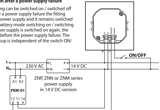
Figure 3. Automatic backup switch on after a power supply failure
