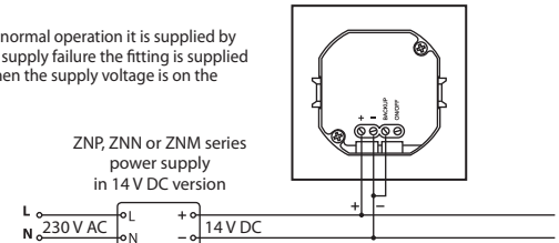
Figure 2. Battery backup with a possibility of manual switch on
