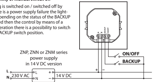
Figure 3. Automatic backup switch on after a power supply failure
