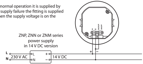
Figure 2. Battery backup with a possibility of manual switch on
