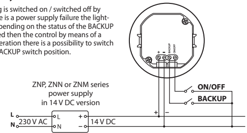
Figure 2. Battery backup with a possibility of manual switch on
