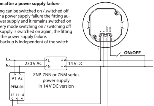
Figure 3. Automatic backup switch on after a power supply failure
